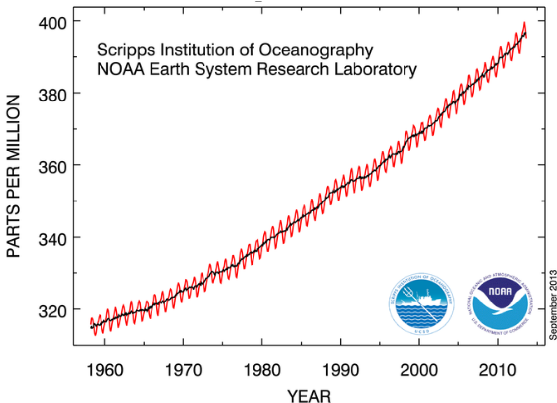
Figure 1. Atmospheric CO 2 record at Mauna Loa Observatory, Hawaii, USA
