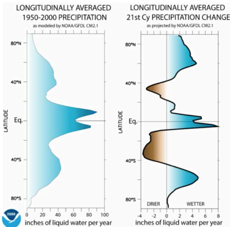
Figure 3. Projected changes in precipitation by latitude
